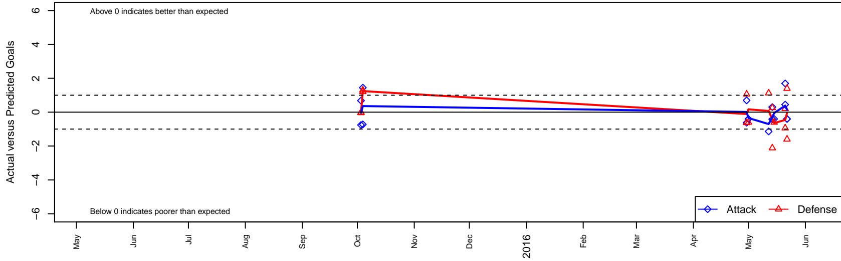
PVSC United Real B04 Dots are actual minus expected GF (blue circles) and GA (red triangles). Blue line is smoothed change in attack strength. Red is smoothed change in defense strength.
